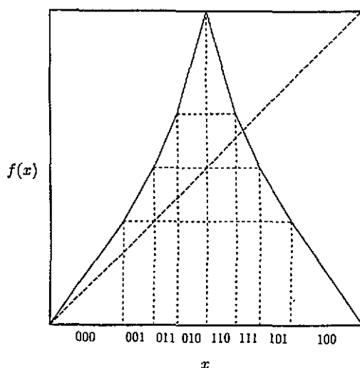
Figure 2. Example of a three-step memory map on X = [0, 1] . For simplicity, we have chosen a symmetric case, although our approach is valid in full generality. The parameters are s(0, 0, 0) = \frac{10}{7} , s(0, 0, 1) = \frac{12}{7} , s(0, 1, 1) = \frac{9}{4} , s(0, 1, 0) = \frac{7}{2} and l(0, 0, 0) = \frac{49}{212} , l(0, 0, 1) = \frac{21}{212} , l(0, 1, 1) = \frac{16}{212} , l(0, 1, 0) = \frac{20}{212} . The general condition for the Markov property of such maps implies the relation s(0, 0, 1)s(0, 1, 0)(s(0, 0, 0) - 1)(s(0, 1, 1) - 1) = s(0, 0, 0)s(0, 1, 1) between the slopes. The length scales follow from normalization.
