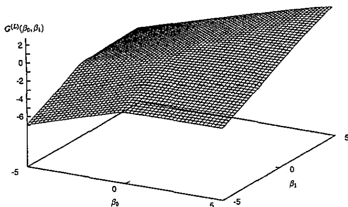
Figure 7. Thermodynamic potential \tilde{G}^{(L)}(\beta_0, \beta_1) of the fully developed logistic map for bivalued periodic test sequences \beta_0, \beta_1, \beta_0, \beta_1, \dots , as computed from the largest eigenvalue of the 'path-integral transfer operator' \mathcal{L}_N .
