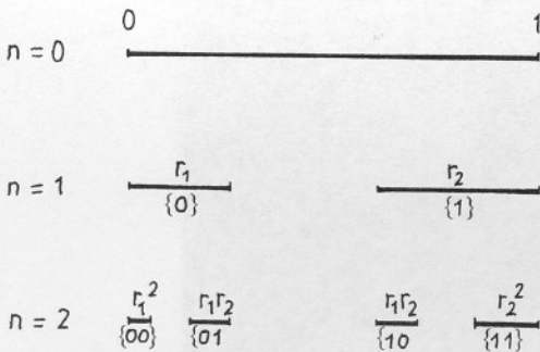
Fig. 8. The first steps in constructing a two-scale Cantor set ( r_1 = 0.25, r_2 = 0.4 ). For the resulting fractal D_0 = 0.611 . The codes associated with the intervals will be explained in Section 14.
