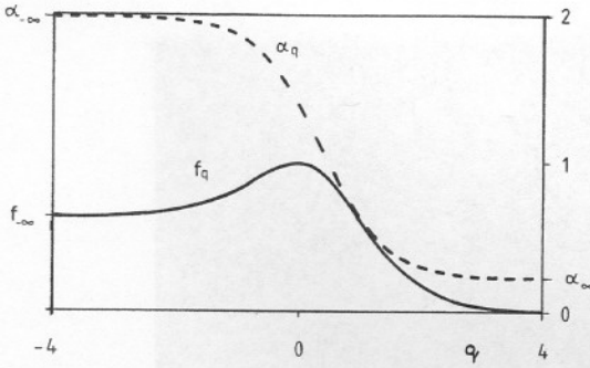
Fig. 15. The q -dependence of the fractal dimension f_q , (32), and of the crowding index \alpha_q , (34), for the multifractal constructed in the previous Figure.
