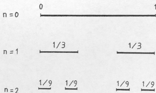
Fig. 2. The first steps in constructing the triadic Cantor set. For the resulting fractal D_0 = 0.631 .
