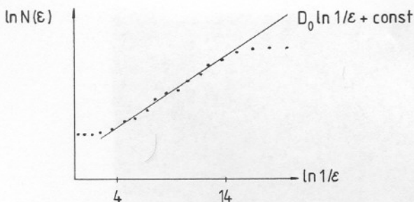
Fig. 3. A typical \ln N(\epsilon) vs. \ln(1/\epsilon) plot.
