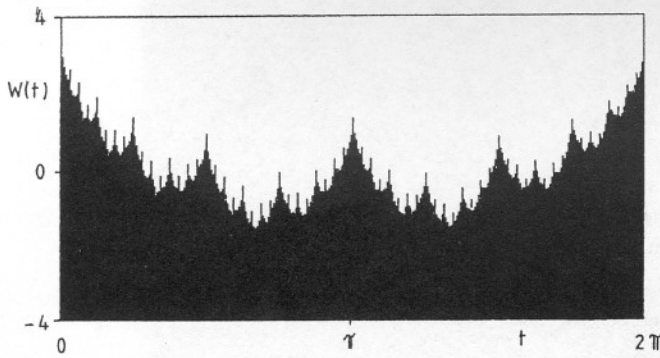
Fig. 11. The Weierstrass function for D = 1.5, \gamma = 2 when it is 2\pi -periodic. The plot was obtained by keeping Fourier components with n \leq 10 in (18). Note that the fractal dimensions of the curves shown on Figs. 10 and 11 are the same.
