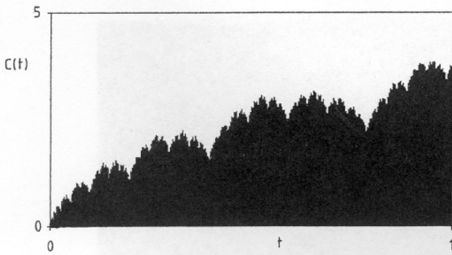
Fig. 10. The Weierstrass-Mandelbrot function for D = 1.5, \gamma = 2 . The plot was obtained by keeping Fourier components with |n| \leq 10 in (14).
