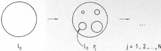
Fig. 7. Schematic construction of a multi-scale fractal.
