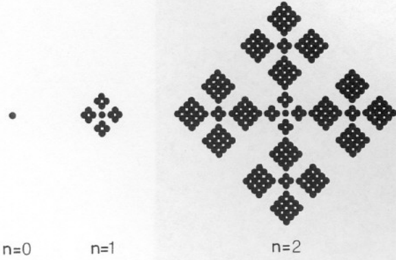
Fig. 9. The first steps in constructing a two-scale snowflake fractal by means of a growth process.
